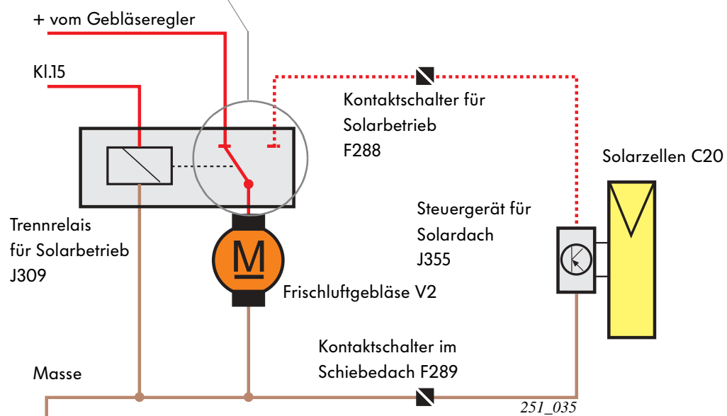
251_035b
